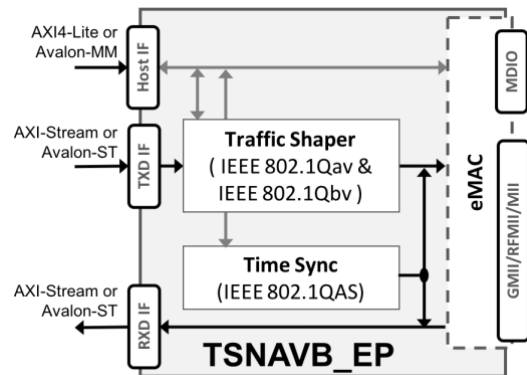
Block diagram showing the major elements of the TSN Ethernet Subsystem IP available from CAST.
